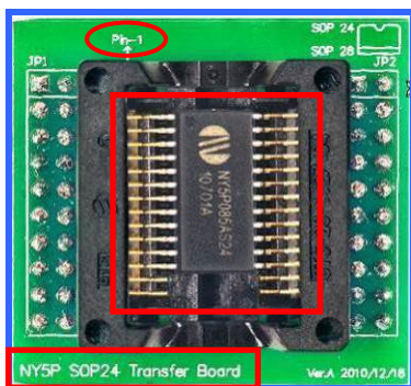
SOP24 Transfer Board
