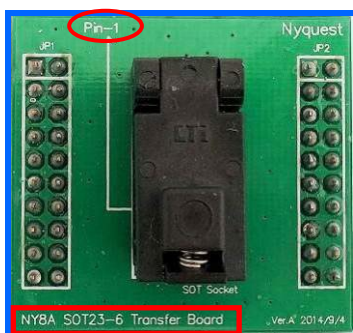
SOT23-6 Transfer Board for NY8A series
