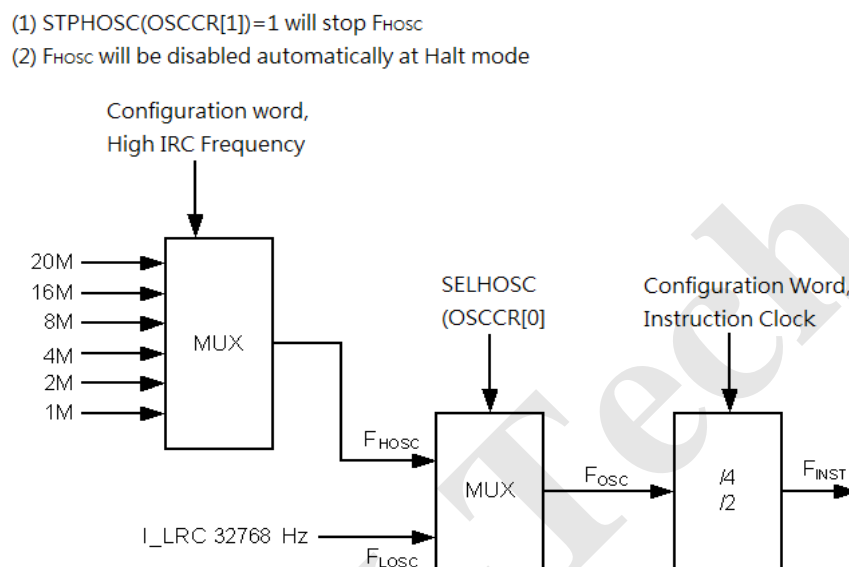
Figure 18 Oscillation Configuration of AT8A513H1
