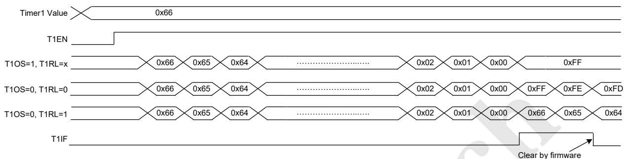
Figure 12 Timer1 Timing Chart
