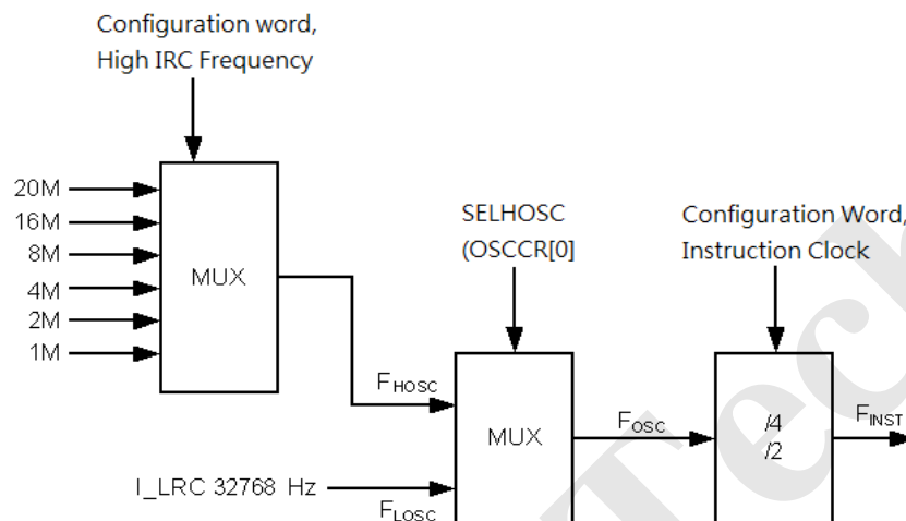
Figure 18 Oscillation Configuration of AT8A513H1
