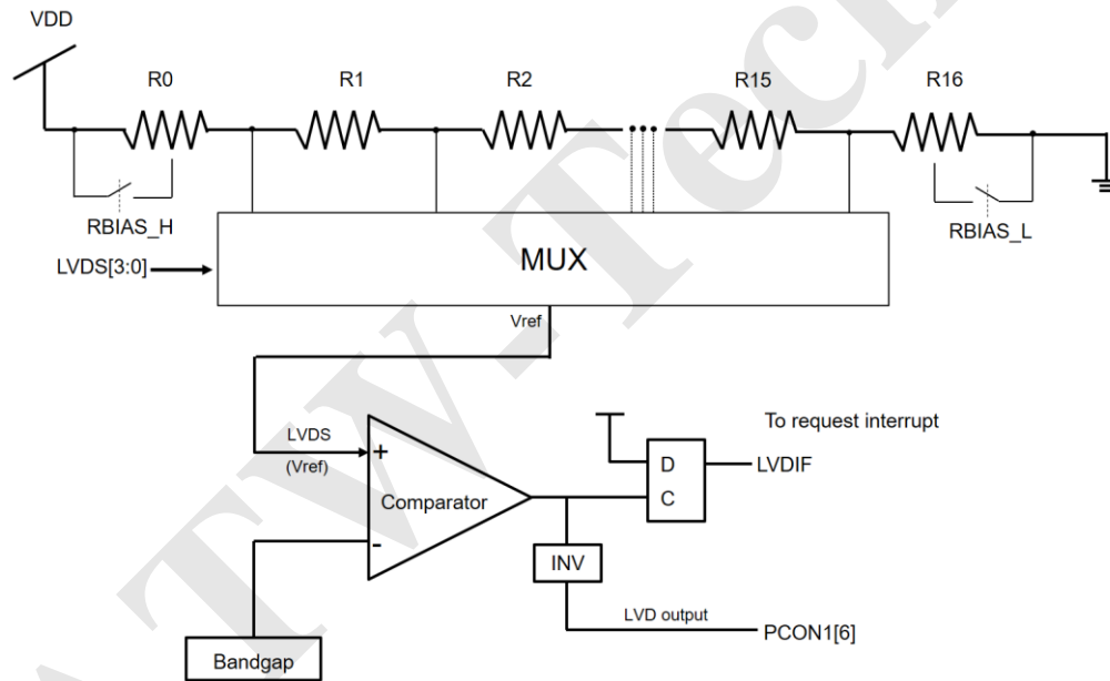
Figure 17 Vref hardware connection &amp; LVD block diagram
