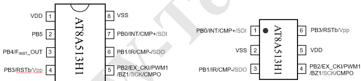
Figure 1 Package pin assignment
