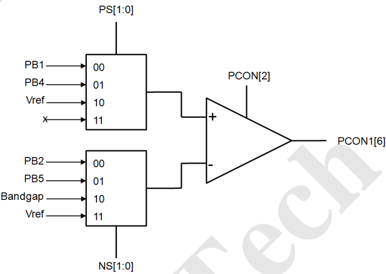
Figure 23 Comparator block diagram
