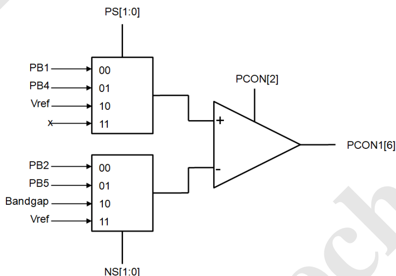
Figure 23 Comparator block diagram
