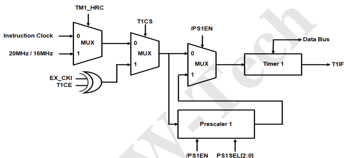
Figure 12 Block Diagram of Timer1
