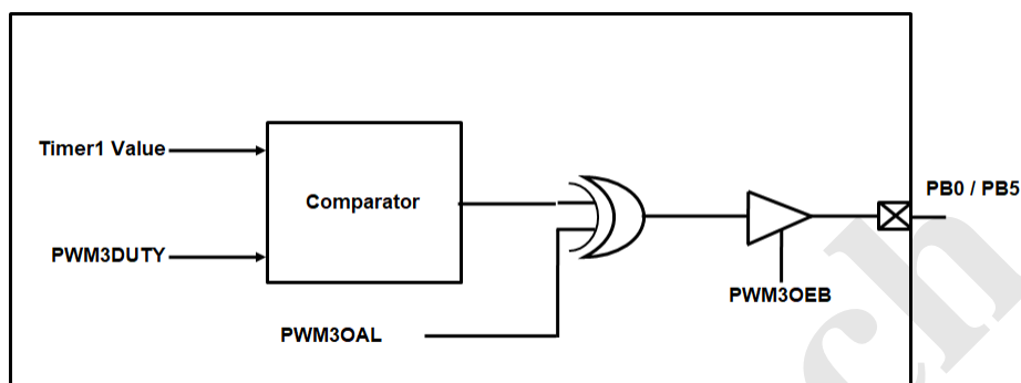
Figure 17 PWM3 Block Diagram
