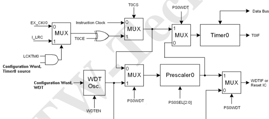
Figure 11 Block Diagram of Timer0 and WDT
