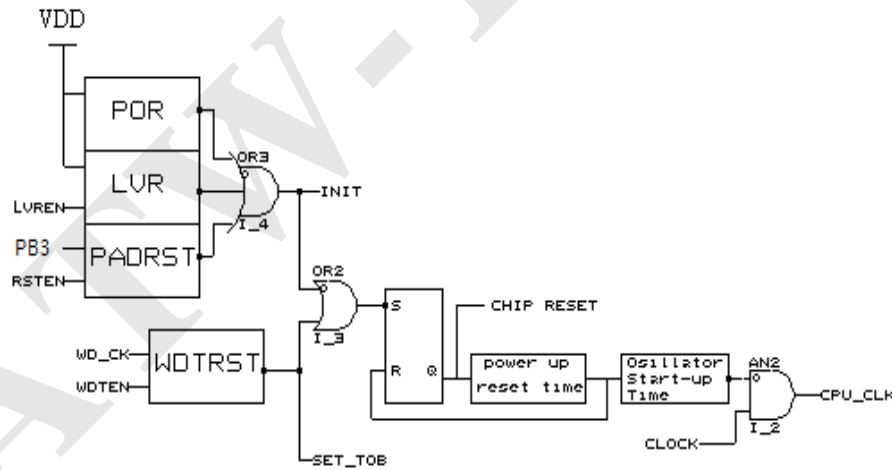
Figure 21 Block diagram of on-chip reset circuit
