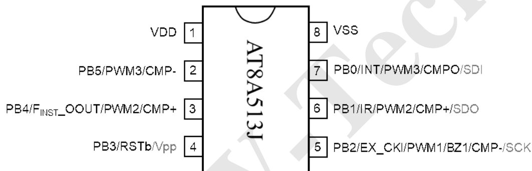
Figure 1 Package pin assignment
