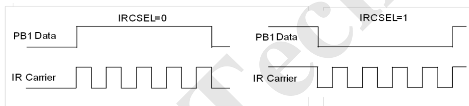
Figure 18 Polarity of IR Carrier vs. Output Data
