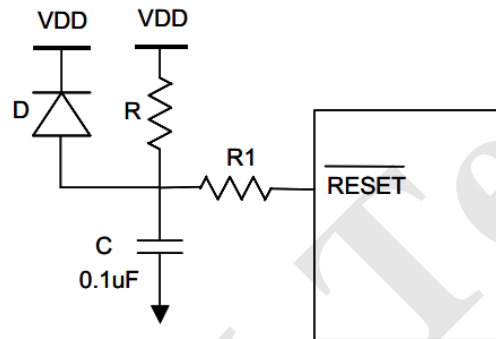
Figure 22 Block Diagram of Reset Application
