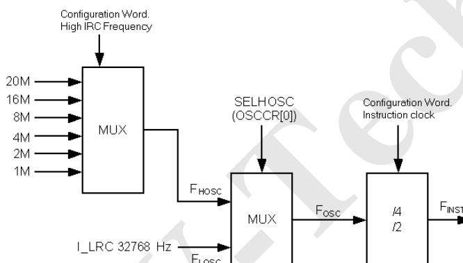
Figure 19 Oscillation Configuration of AT8A513J
