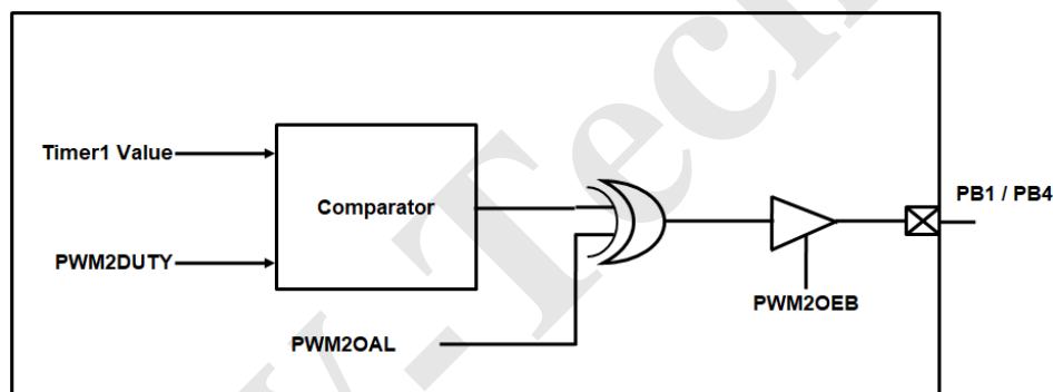
Figure 16 PWM2 Block Diagram
