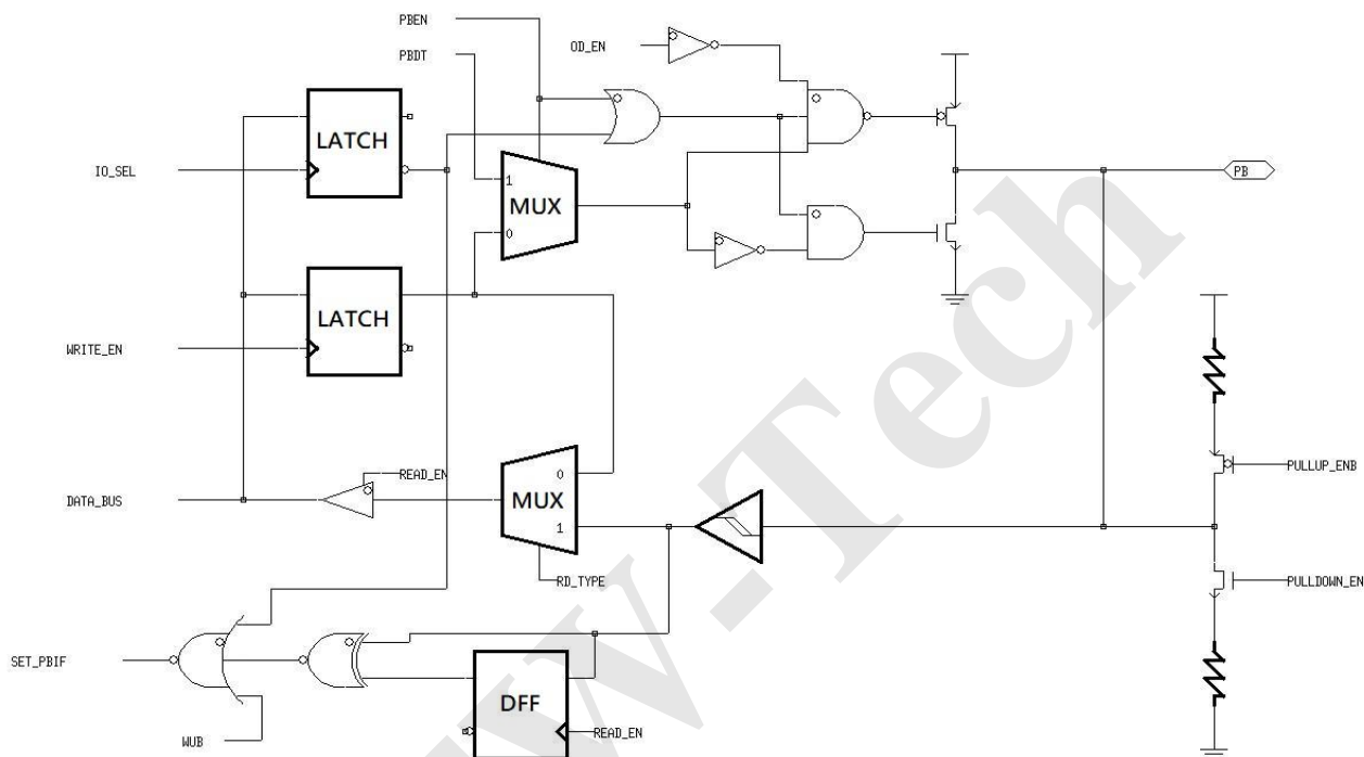
Figure 5 Block Diagram of PB0
