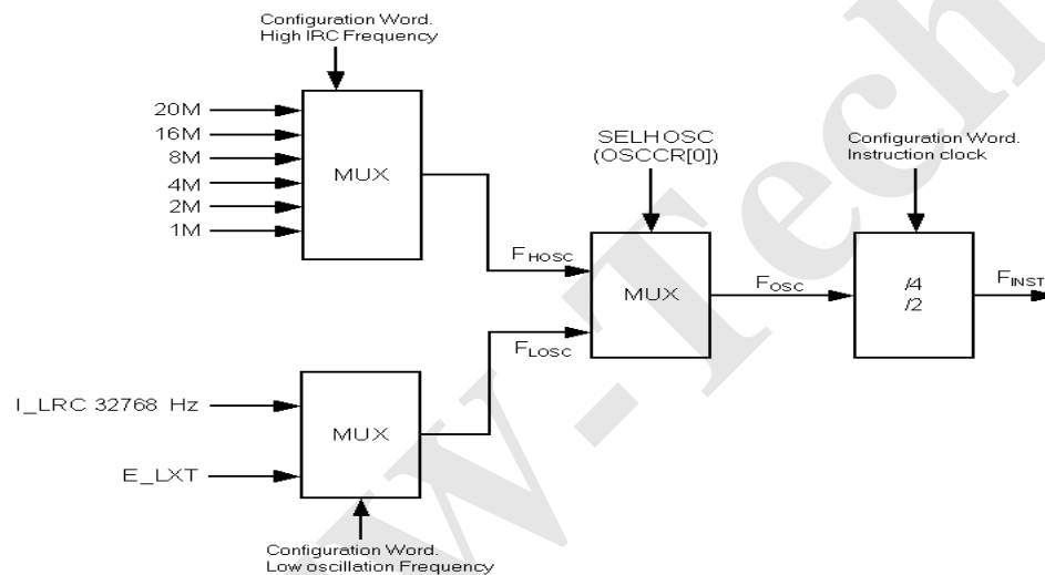
Figure 19 Oscillation Configuration of AT8A513L
