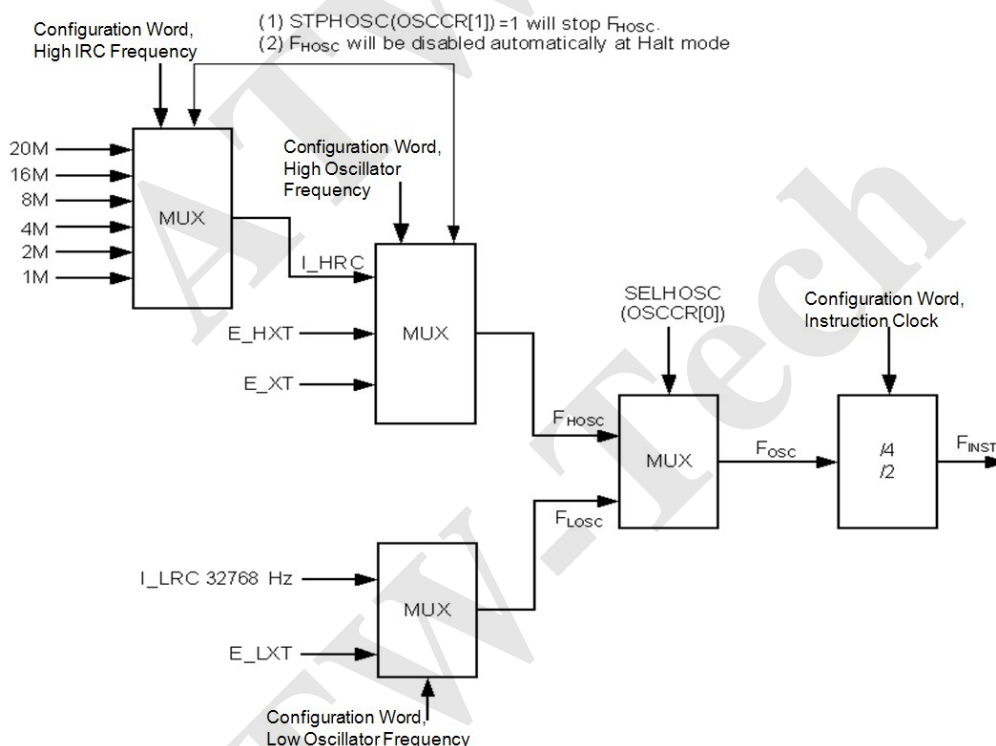
Figure 18 Oscillation Configuration of AT8A53B
