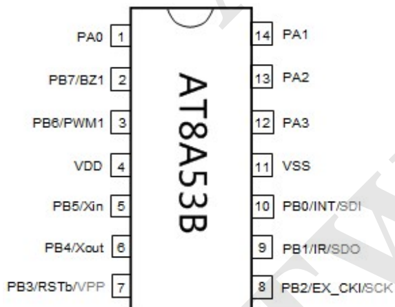
Figure 1 Package pin assignment
