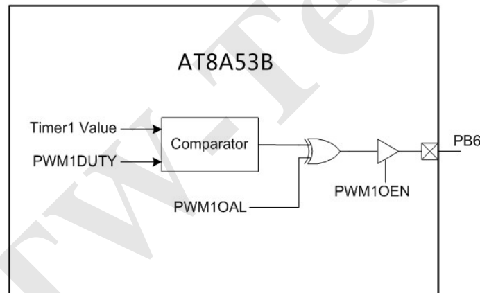
Figure 15 PWM1 Block Diagram
