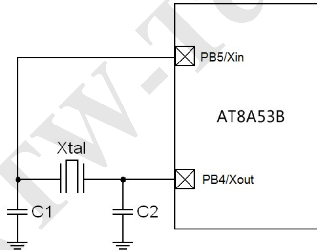
Figure 19 Connection for External Crystal Oscillation
