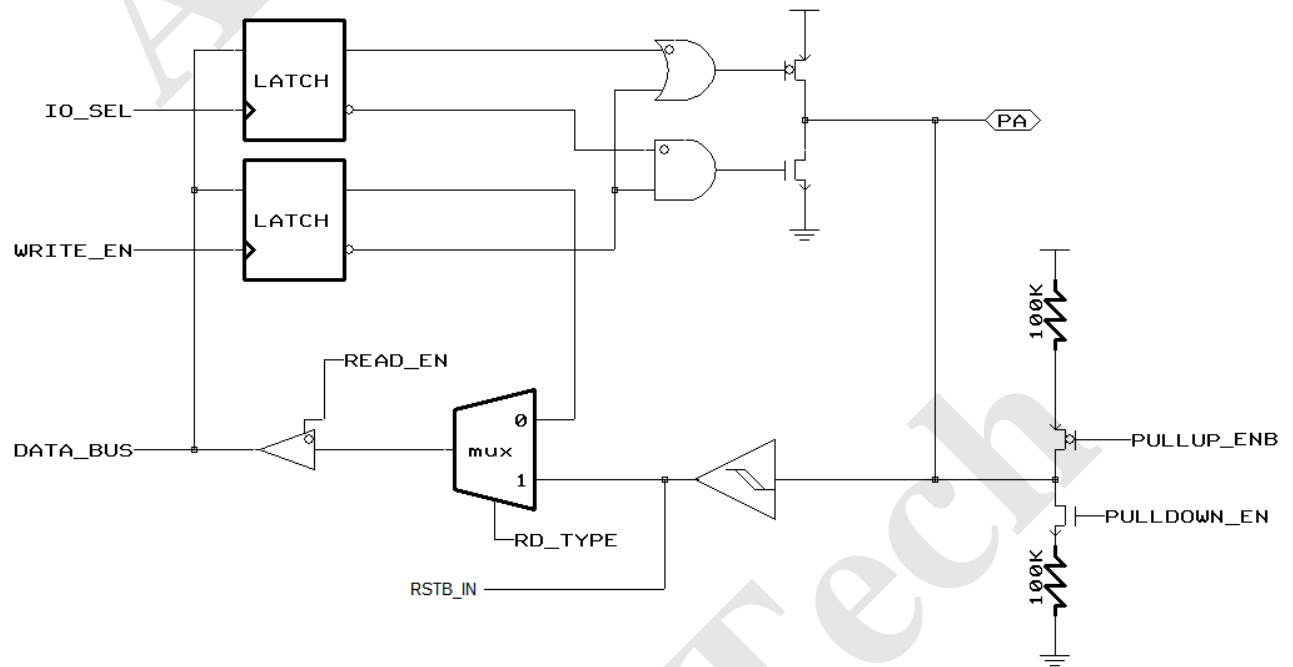
Figure 9 Block Diagram of PA5
