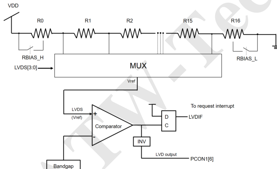
Figure 32 Vref hardware connection & LVD block diagram
