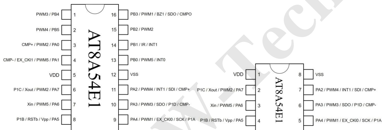
Figure 1 Package pin assignment
