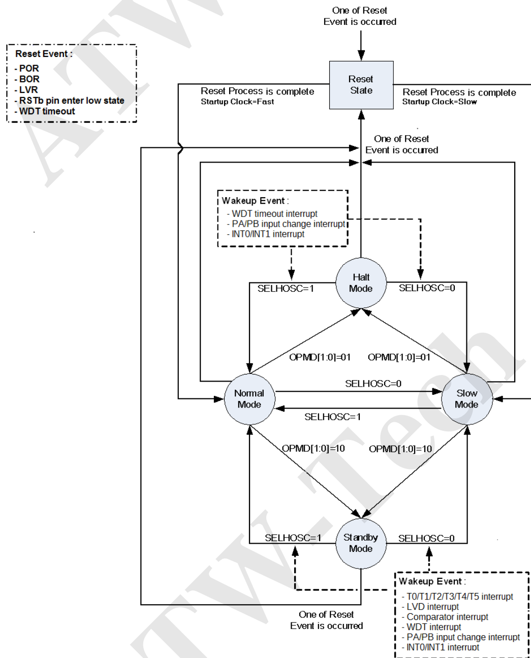
Figure 35 Four Operating Modes
