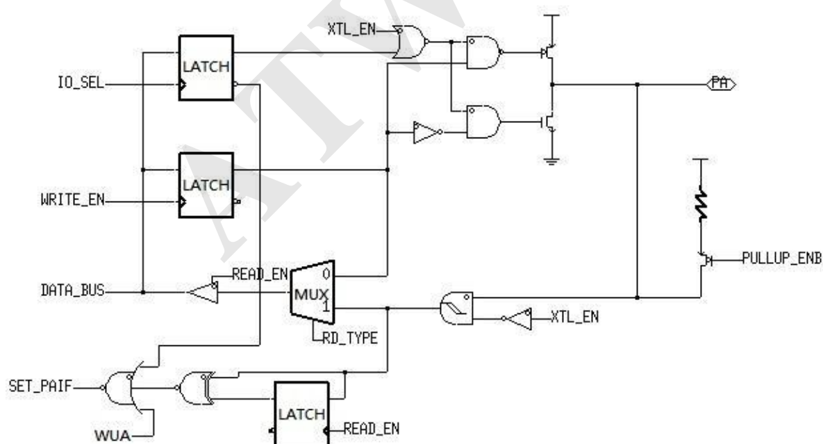
Figure 9 Block Diagram of PA6
