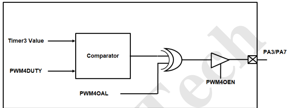
Figure 28 PWM4 Block Diagram
