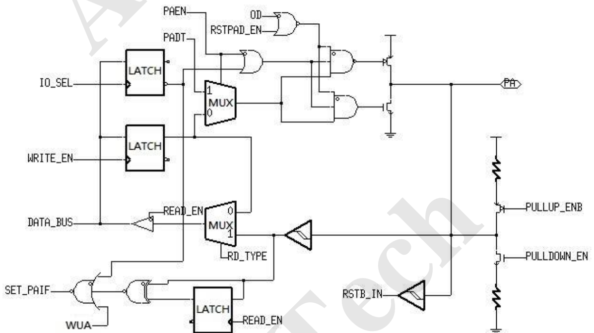
Figure 8 Block Diagram of PA5
