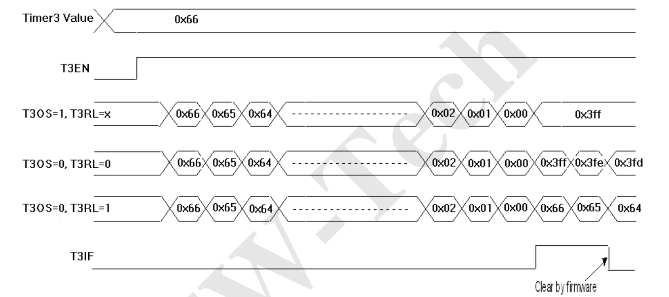
Figure 25 Timer3 Timing Chart
