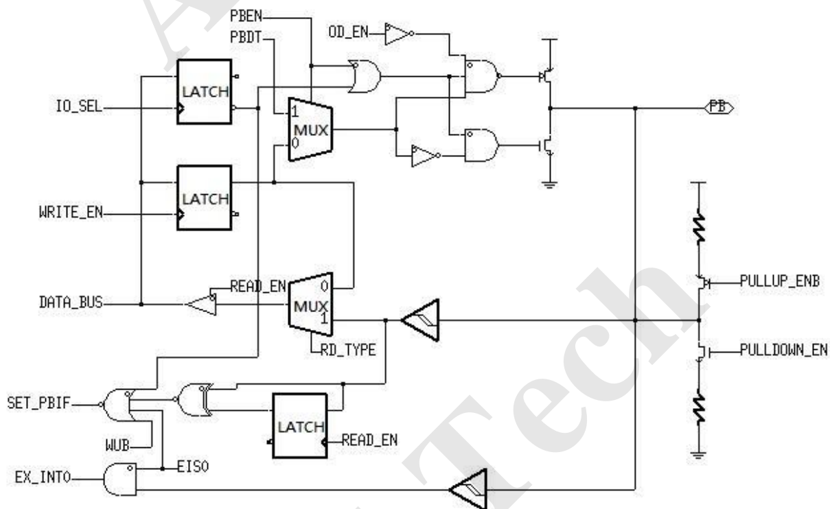
Figure 10 Block Diagram of PB0
