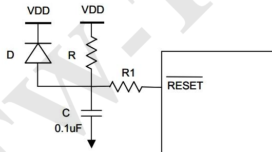
Figure 38 Block Diagram of Reset Application
