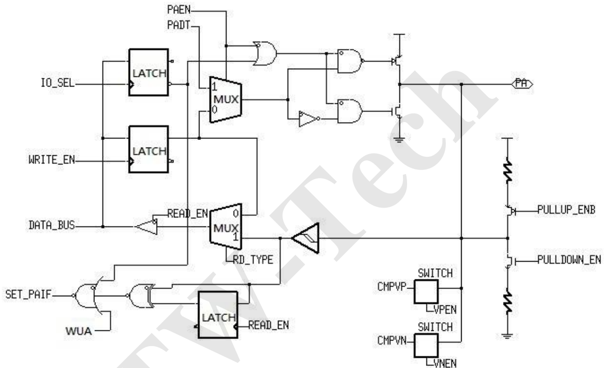
Figure 5 Block Diagram of PA[3:2]&PA0
