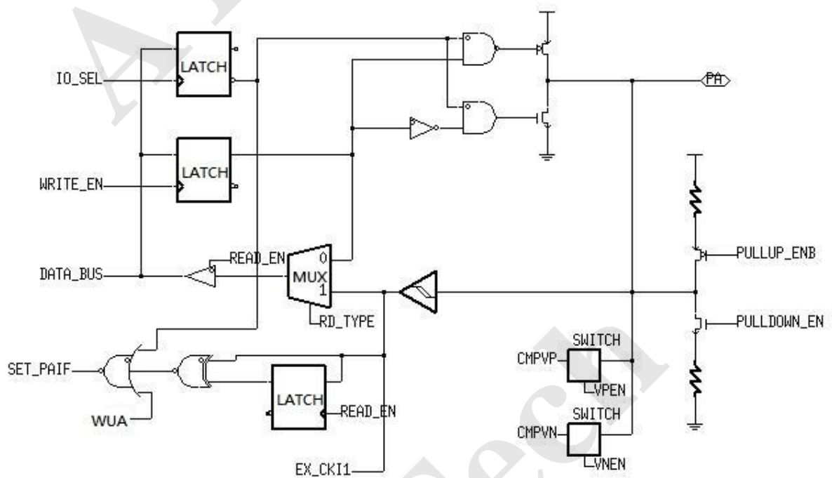
Figure 6 Block Diagram of PA1
