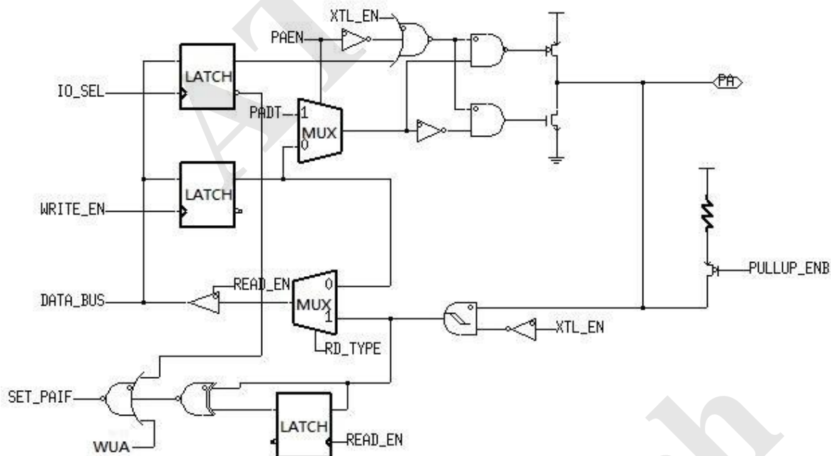
Figure 10 Block Diagram of PA7
