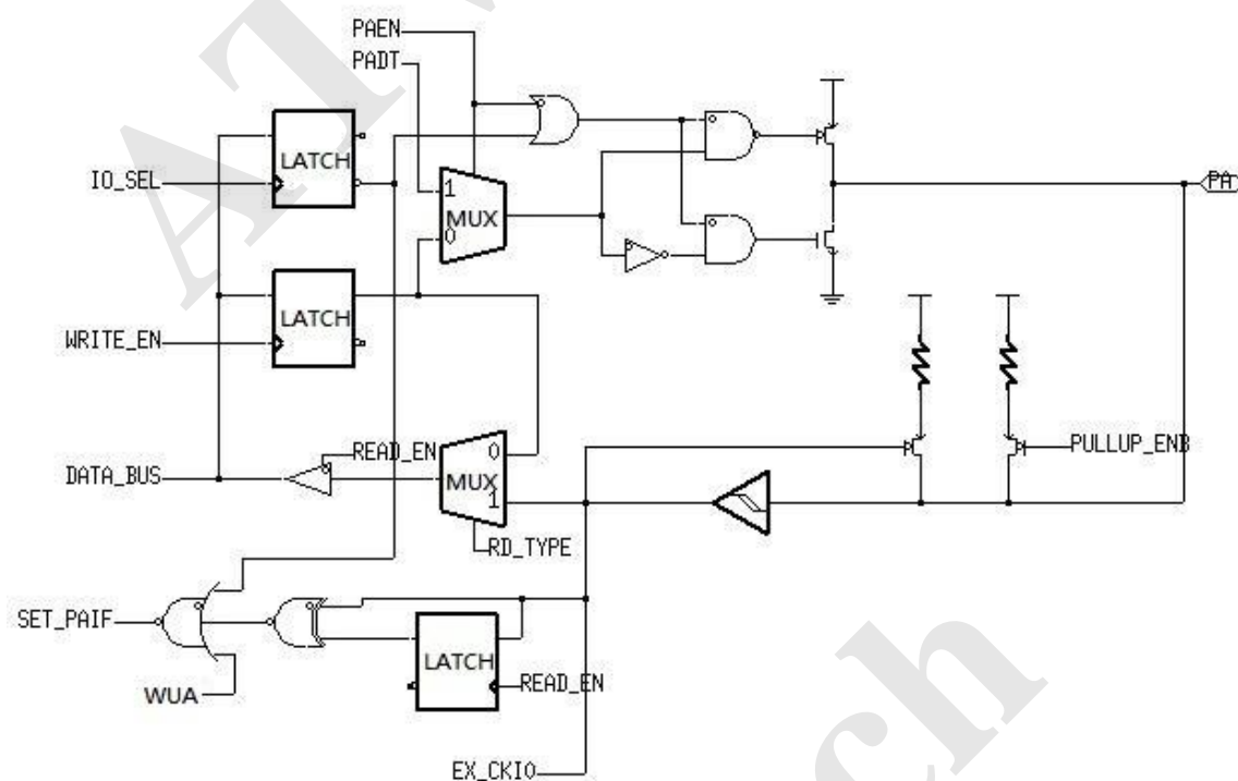
Figure 7 Block Diagram of PA4
