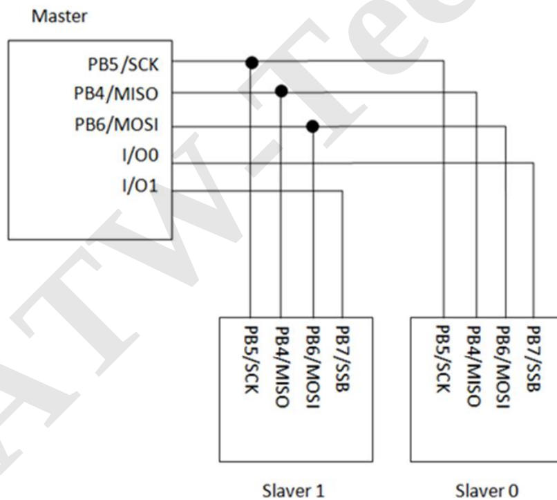
Figure 44 Single Master and Multi Slaves
