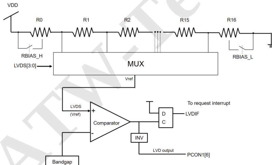
Figure 35 Vref Hardware Connection
