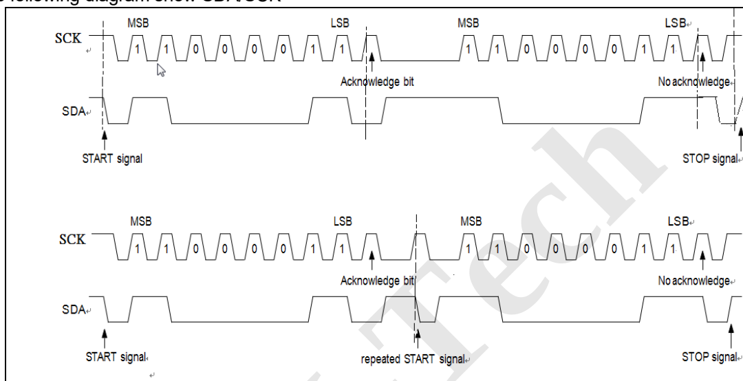
Figure 50 I 2 C Bus Transmission Signal Diagram
