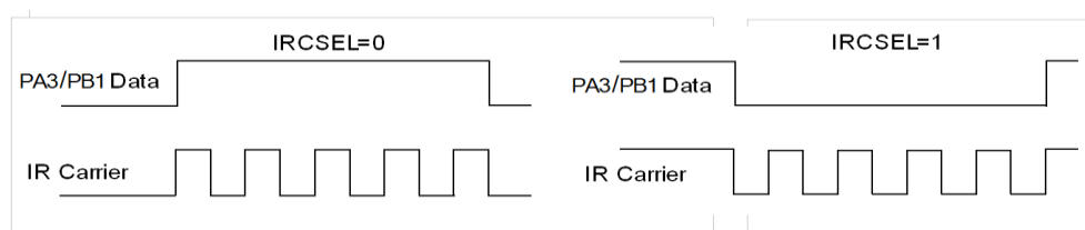
Figure 32 Polarity of IR Carrier vs. Output Data
