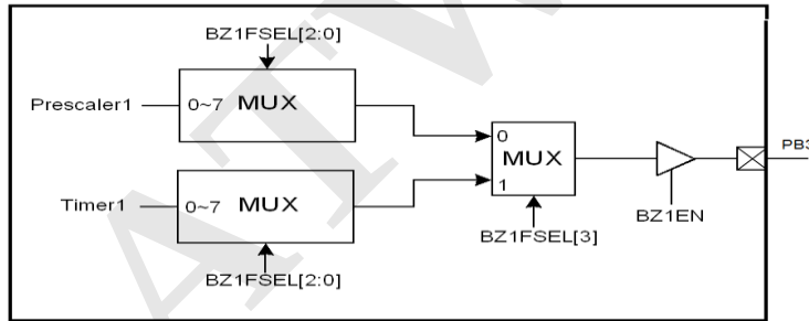
Figure 31 Buzzer1 Block Diagram
