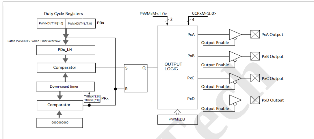
Figure 23 Simplified Block Diagram of Enhanced PWM Mode
