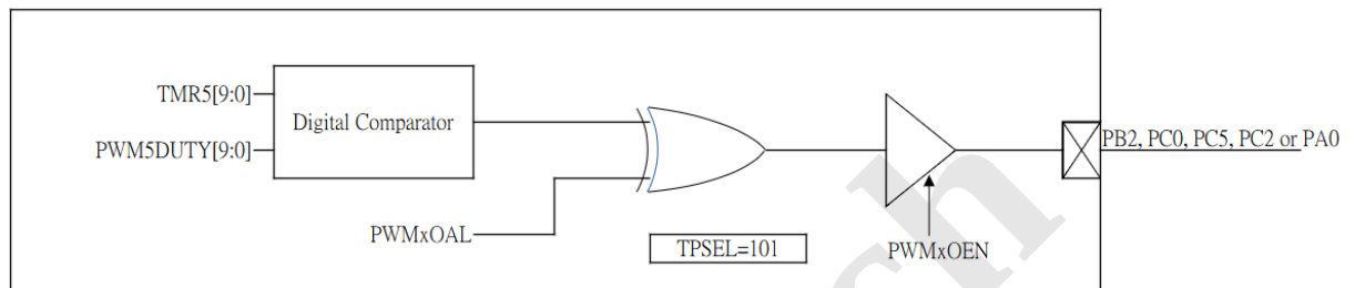
Figure 18 PWM5 Block Diagram
