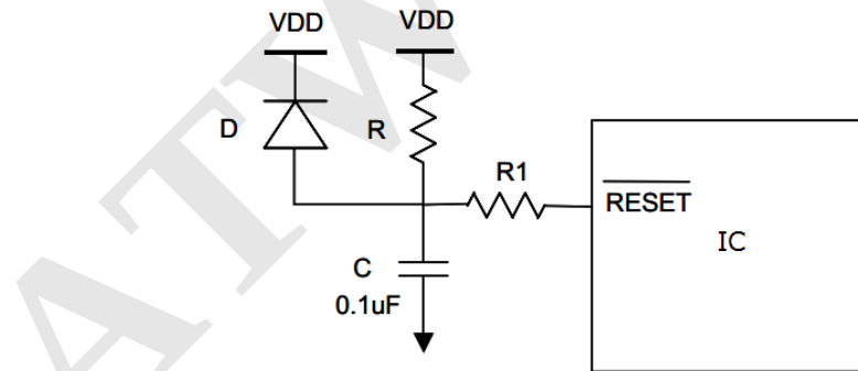
Figure 42 Block Diagram of Reset Application
