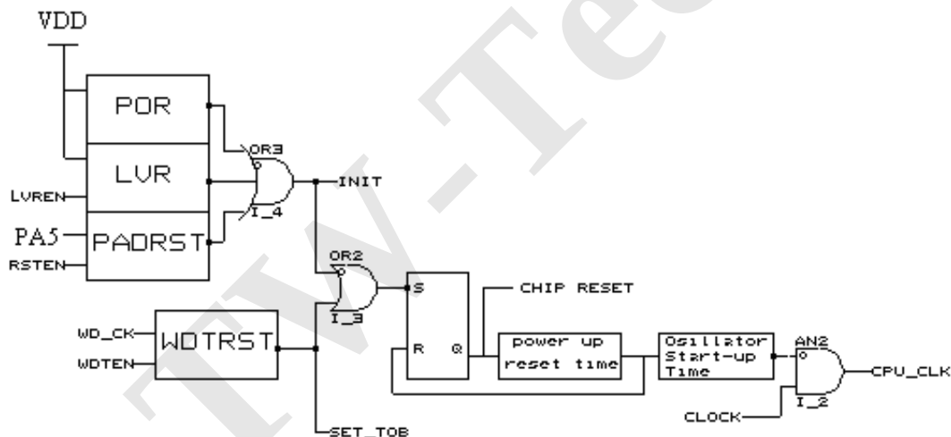
Figure 41 Block diagram of On-Chip Reset Circuit
