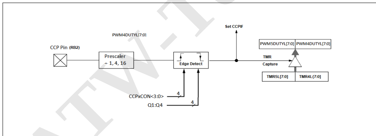
Figure 19 Capture Mode Block Diagram
