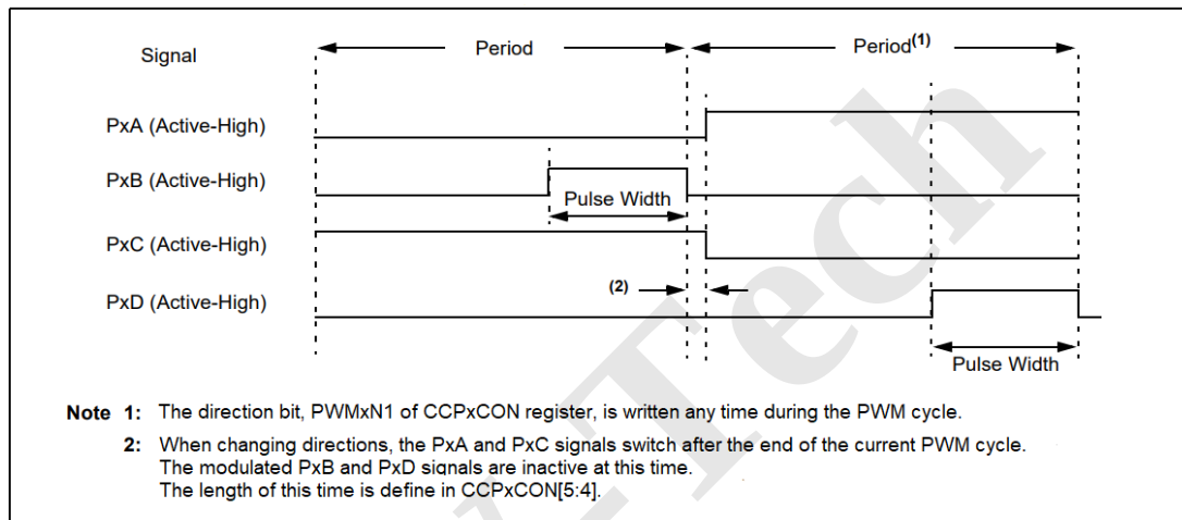
Figure 29 Example of PWM Direction Change
