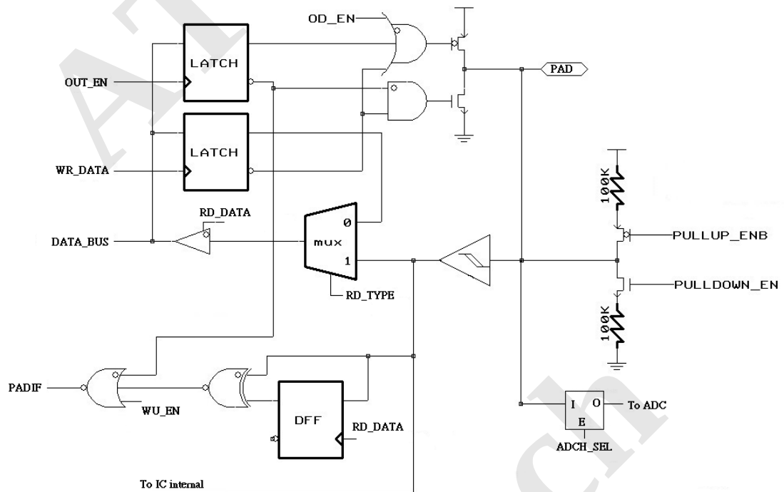
Figure 10 Block Diagram of PB0~PB2, PC0~1
