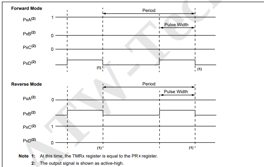
Figure 27 Example of Full-Bridge PWM Output
