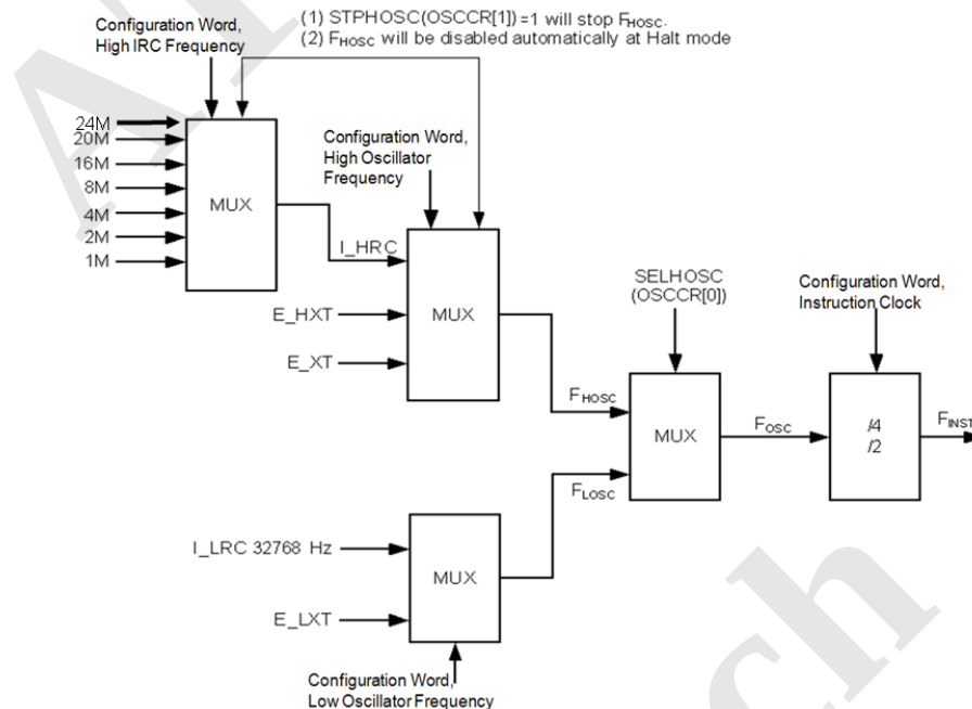
Figure 38 Oscillation Configuration of AT8F2481
