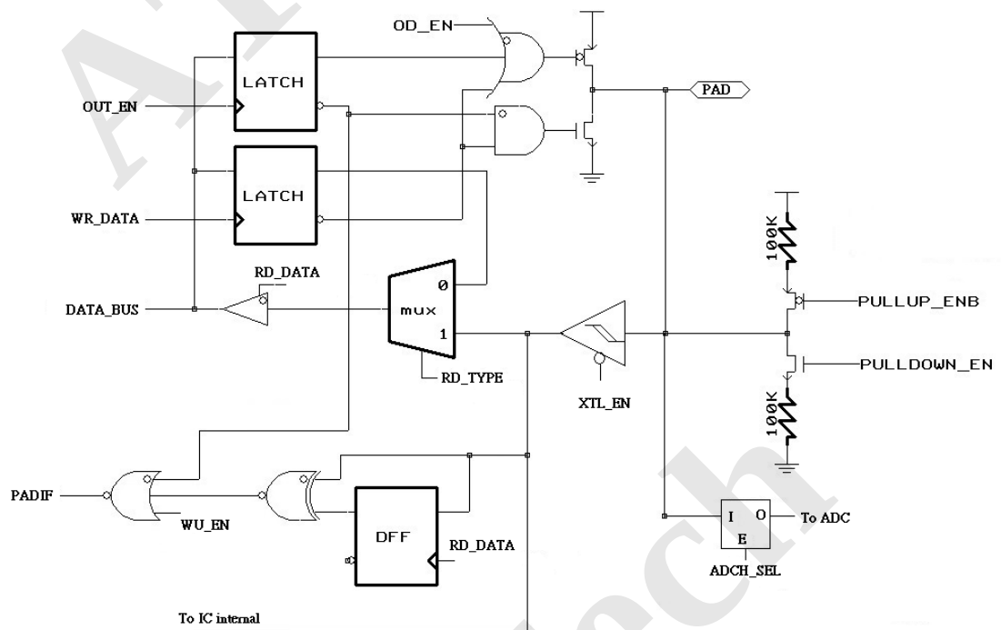
Figure 8 Block Diagram of PA6, PA7
