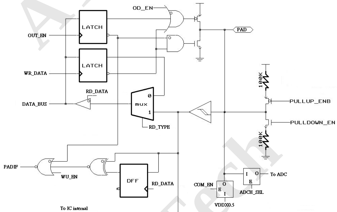
Figure 9 Block Diagram of PB4~PB7, PC2~PC5
