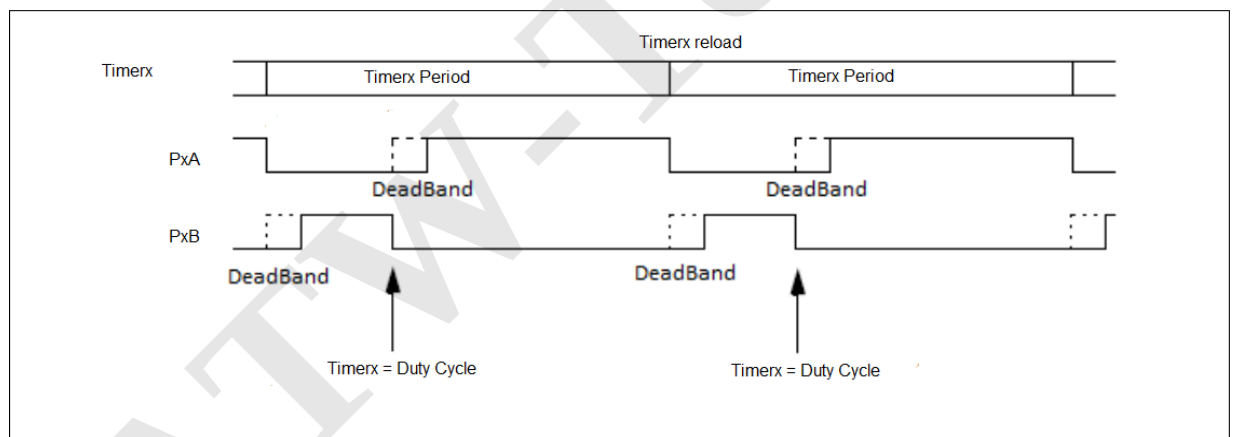
Figure 25 Example of Half-Bridge PWM Output
