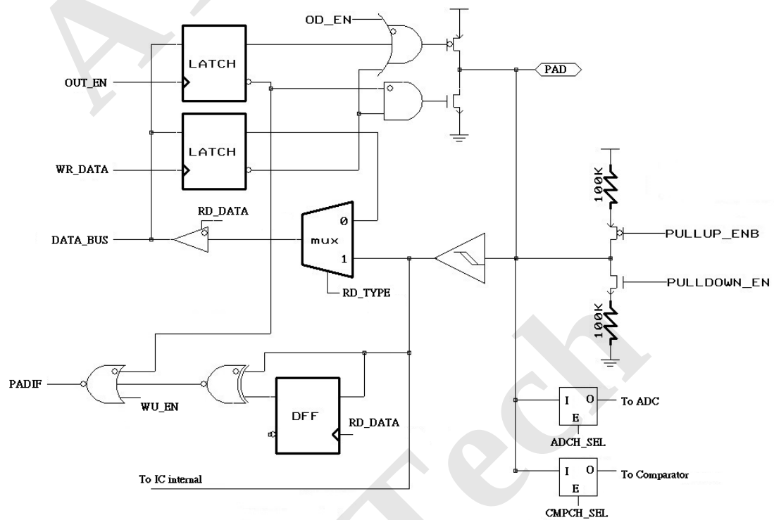
Figure 6 Block Diagram of PA0~PA4, PB3
