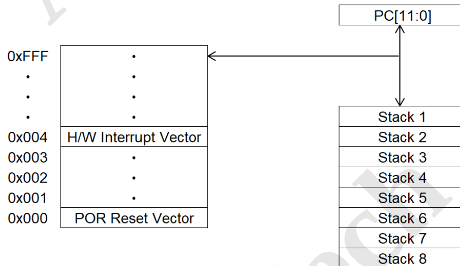
Figure 1 Program Memory Address Mapping
