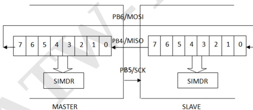
Figure 43 Single Master / Slave
