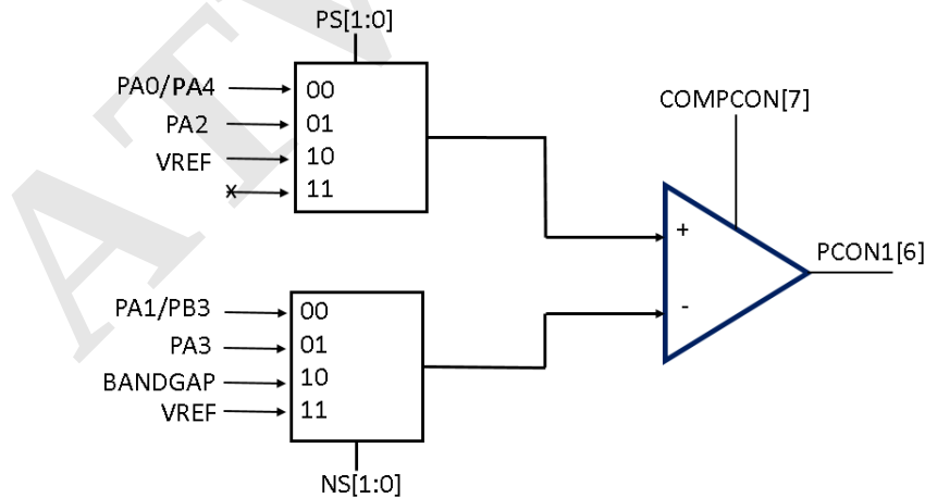
Figure 34 Comparator Hardware Connection
