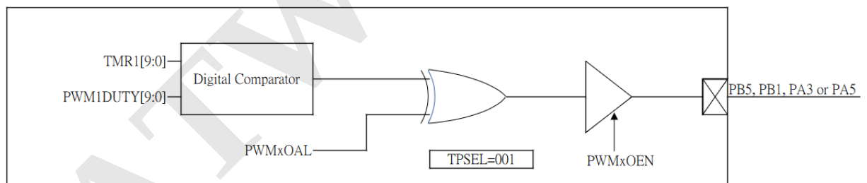
Figure 14 PWM1 Block Diagram
