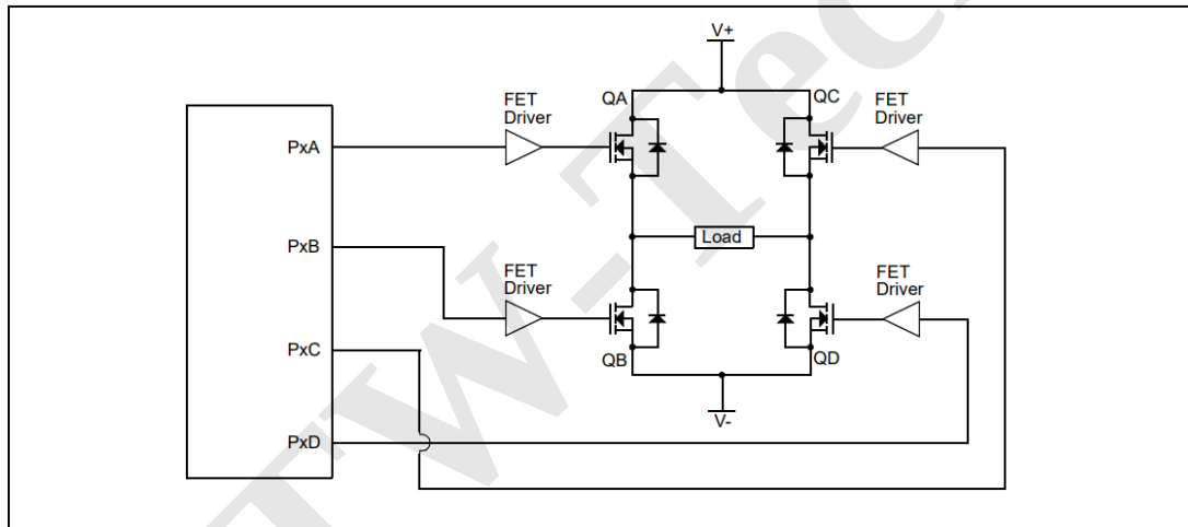
Figure 28 Example of Full-Bridge Applications
