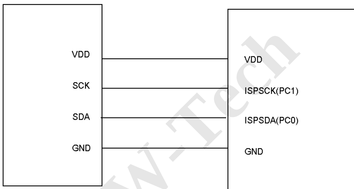
Figure 1 Typical Connection for ISP Programming
