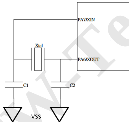
Figure 39 Connection for External Crystal Oscillation
