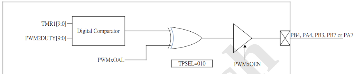
Figure 15 PWM2 Block Diagram
