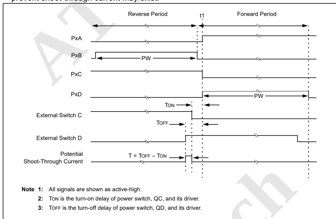
Figure 30 Example of PWM Direction Change at Near 100% Duty Cycle
