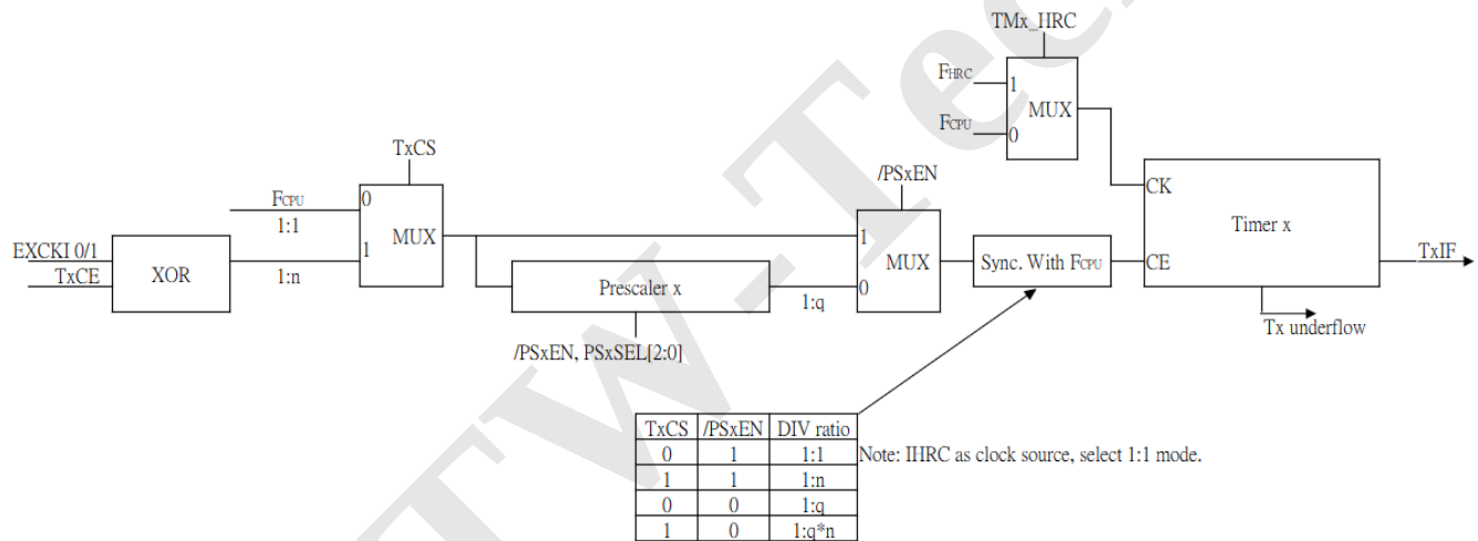
Figure 12 Block Diagram of Timer1 / 4 / 5
