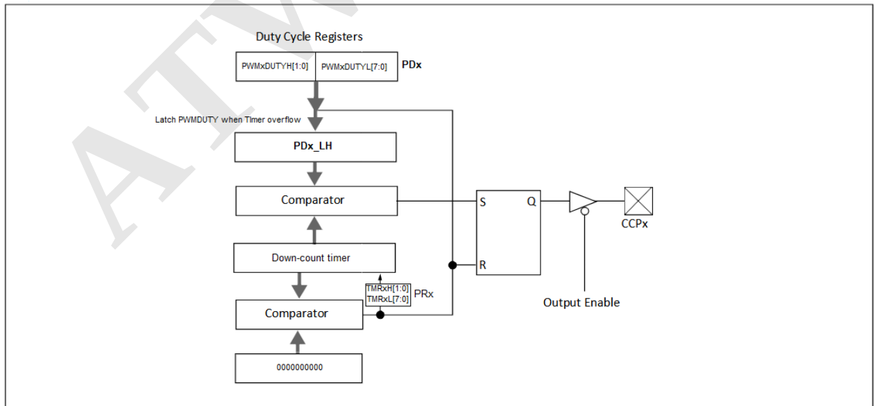
Figure 21 Enhanced PWM Block Diagram
