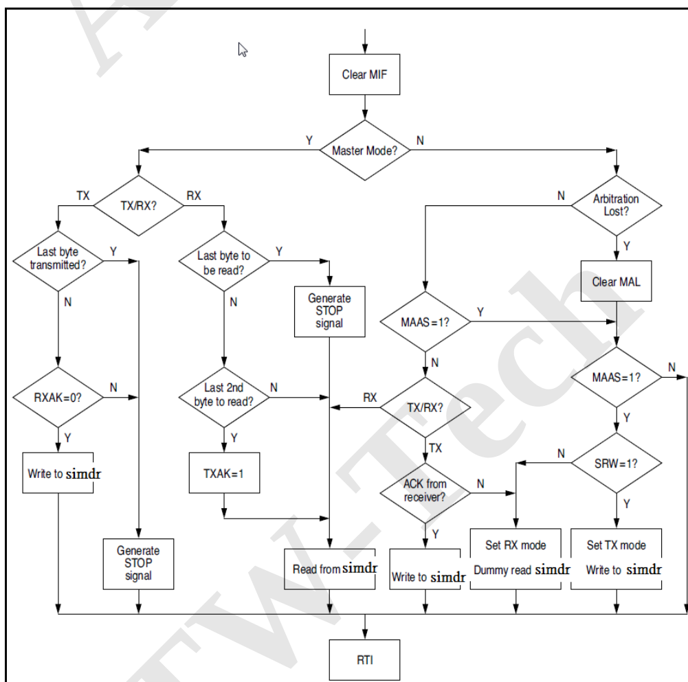
Figure 51 Flowchart of I 2 C Interface Routine
