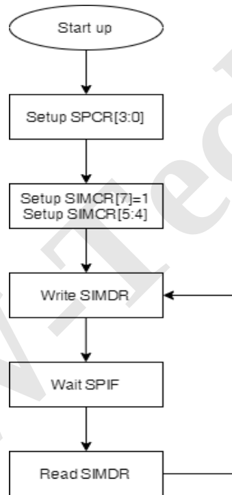
Figure 47 Flowchart of SPI Interface
