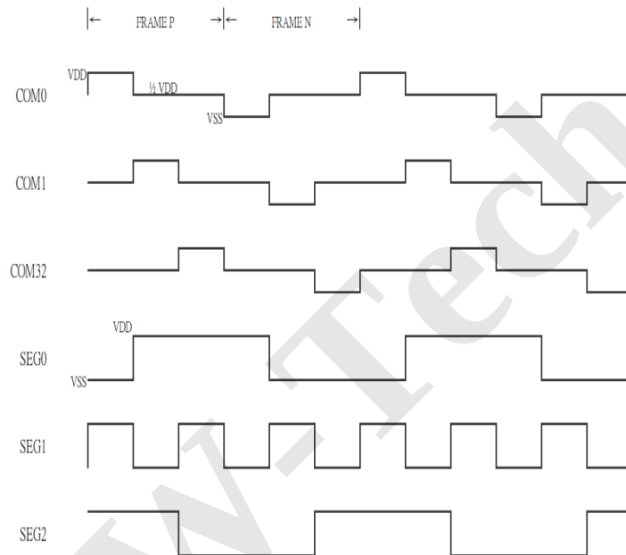
Figure 52 LCD Waveform
