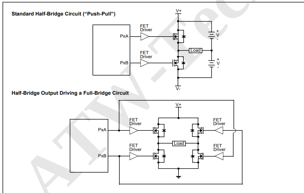
Figure 26 Example of Half-Bridge Applications
