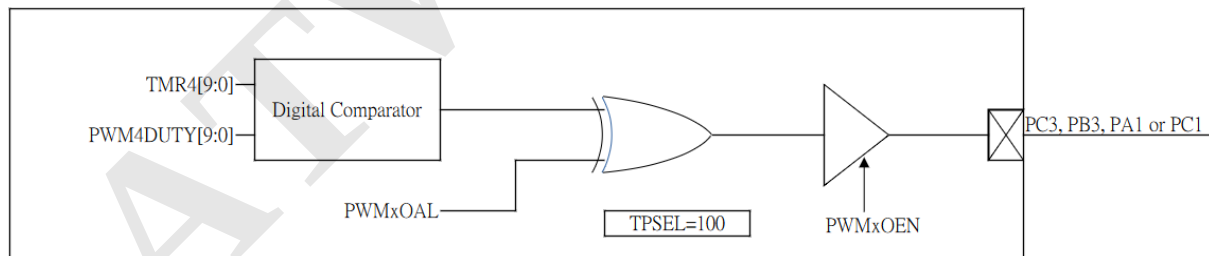
Figure 17 PWM4 Block Diagram
