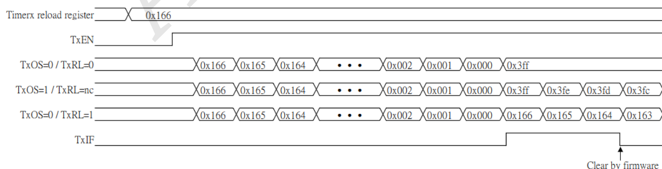
Figure 13 Timer1 / 4 / 5 Timing Chart
