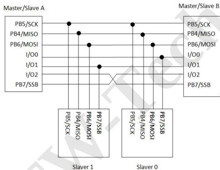
Figure 45 Multi Masters and Multi Slaves
