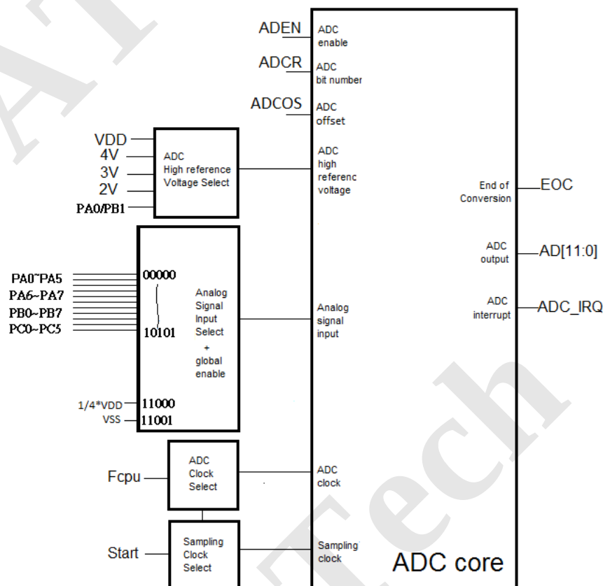
Figure 36 ADC Block Diagram
