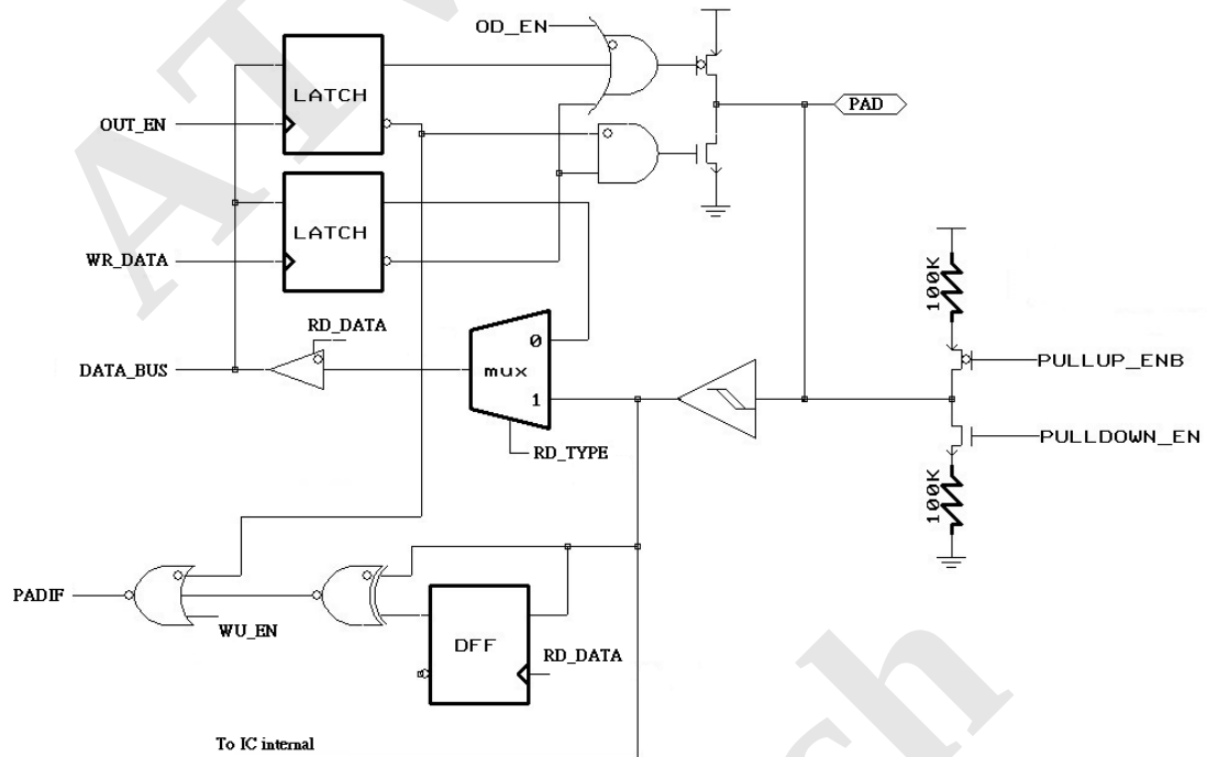
Figure 7 Block Diagram of PA5
