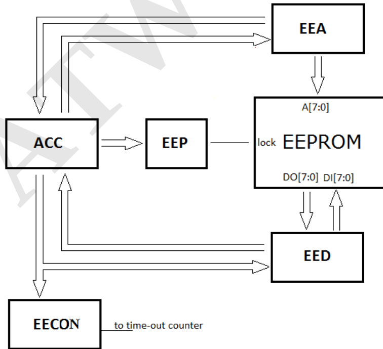
Figure 5 EEPROM Data Access
