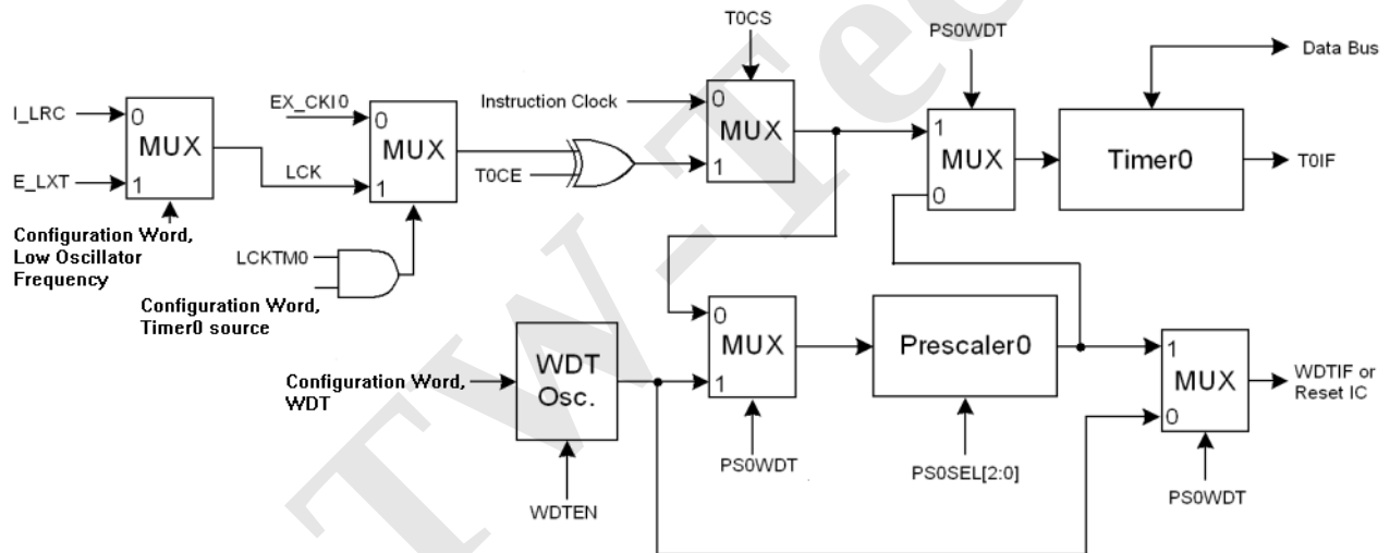
Figure 11 Block Diagram of Timer0 and WDT
