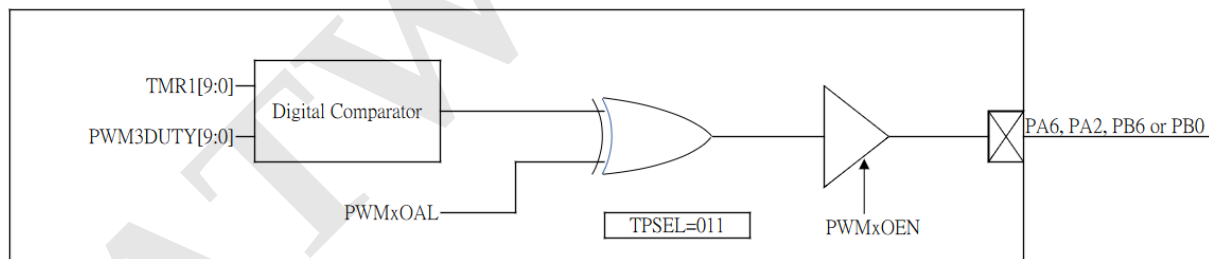
Figure 16 PWM3 Block Diagram
