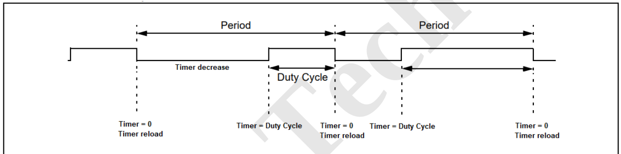
Figure 22 Enhanced PWM Output
